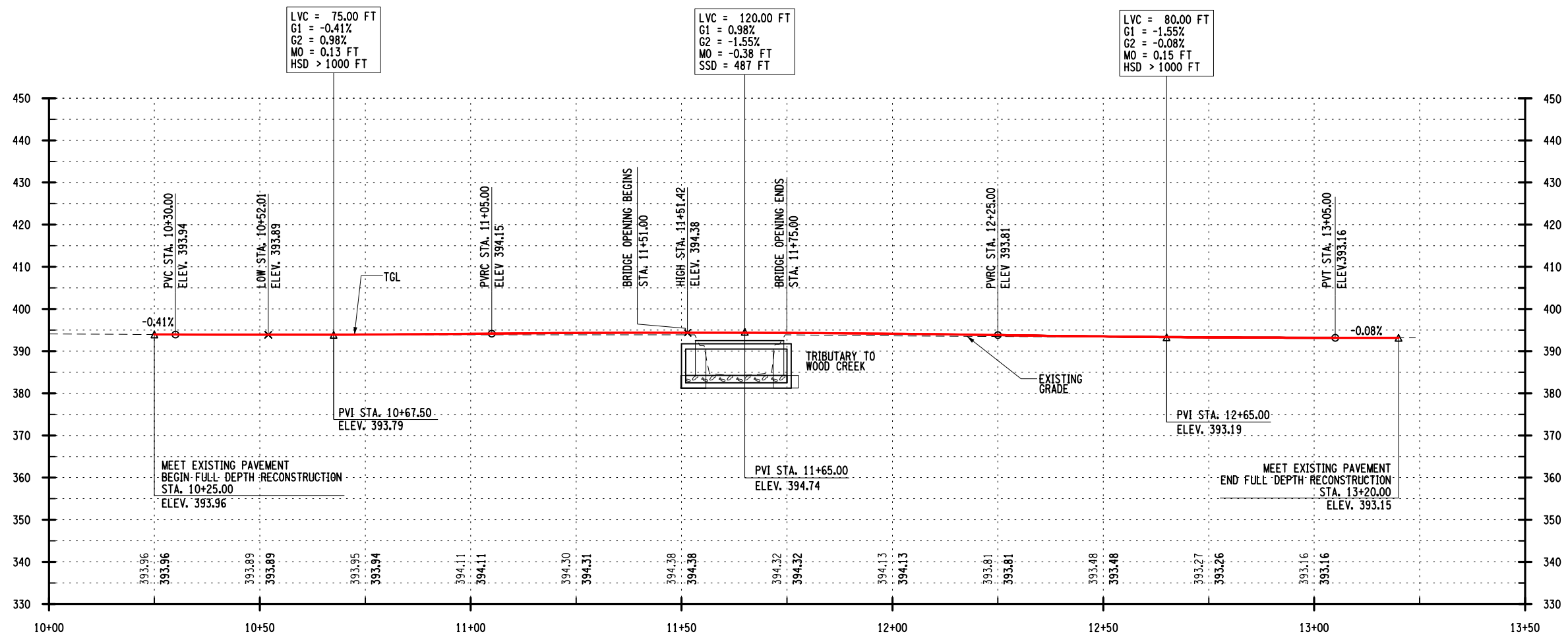
WOOD CREEK ROAD PROFILE
